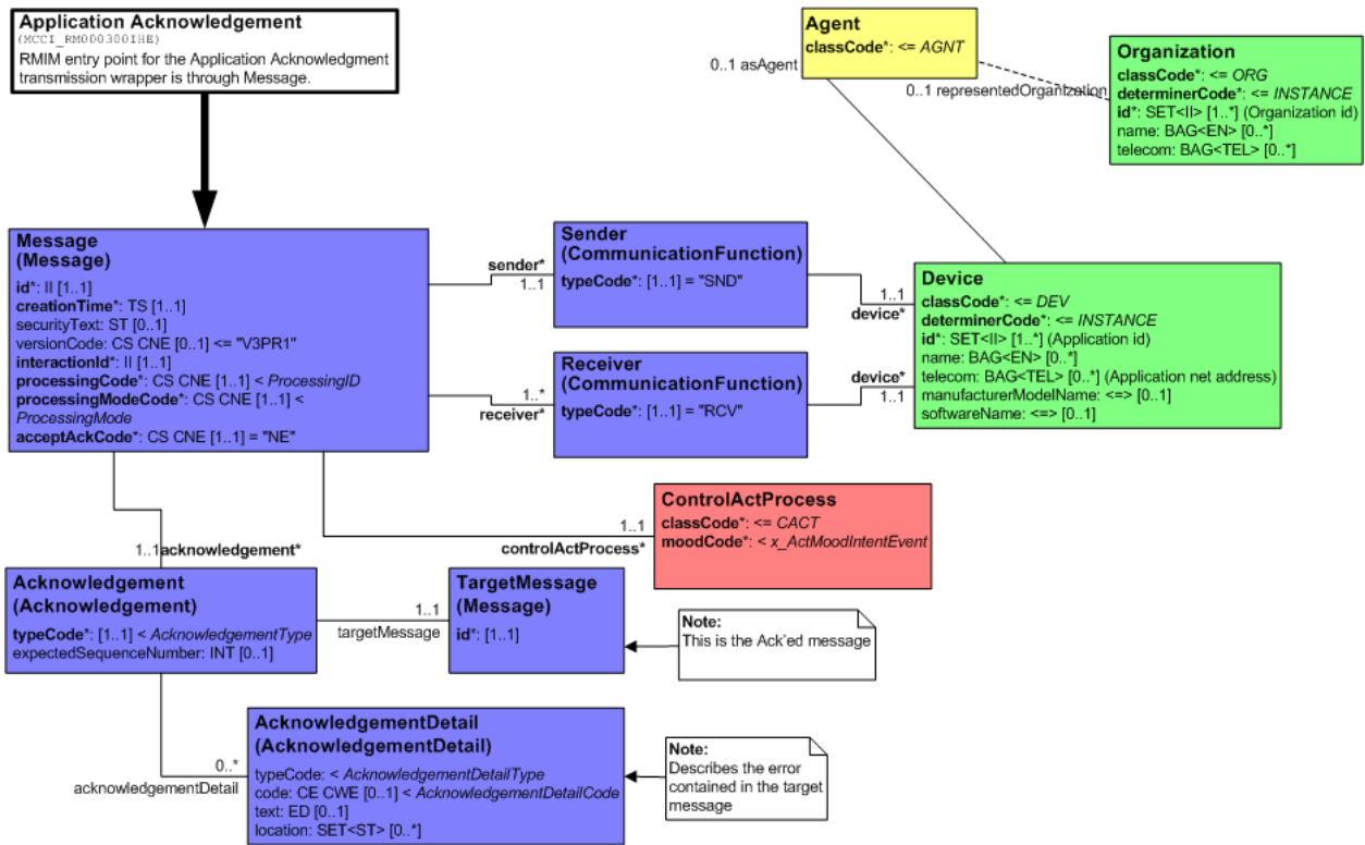
Figure O.1.3-2: Message Information Model
