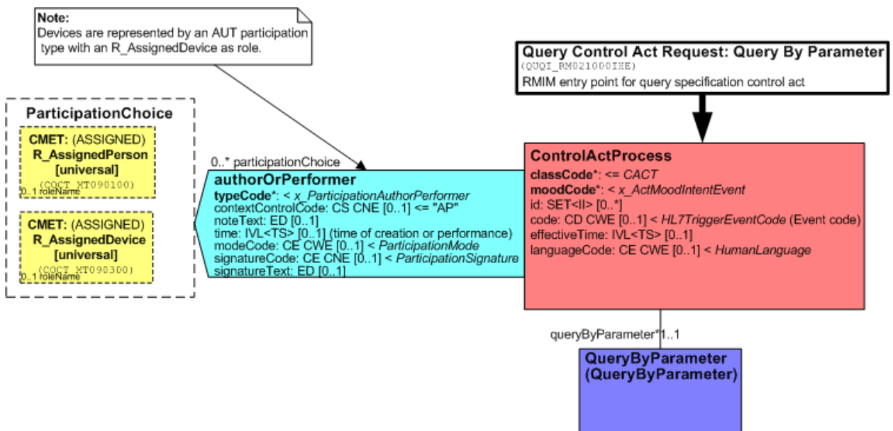
Figure O.2.3-3: Message Information Model
